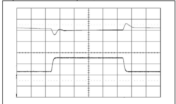
Output voltage response to load current step-change (3-9-3 A) at: T_{P1} = +25^{\circ}\text{C} , V_I = 12\text{ V} , V_O = 3.3\text{ V} , di/dt = 2\ \text{A}/\mu\text{s} , f_{sw} = 320\ \text{kHz} , C_O = 470\ \mu\text{F}/10\ \text{m}\Omega . Default PID Control Loop and NLR. Top trace: output voltage (200 mV/div.). Bottom trace: load current (5 A/div.). Time scale: (0.1 ms/div.).
