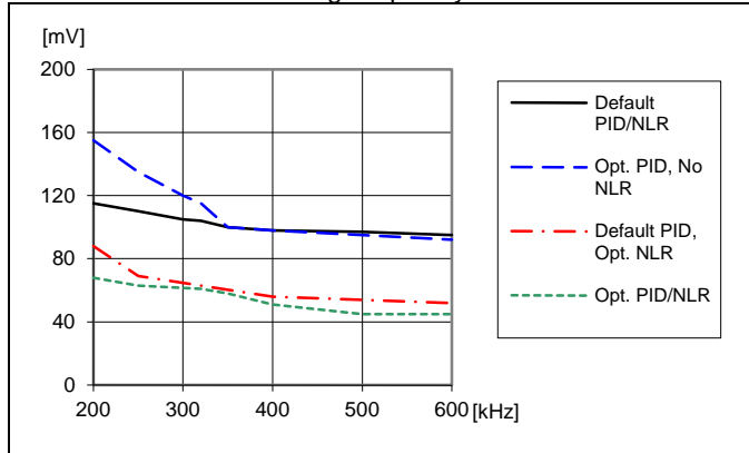
Load transient peak voltage deviation vs. frequency. Step-change (3-9-3 A). T_{P1} = +25^{\circ}\text{C} . V_I = 12\text{ V} , V_O = 3.3\text{ V} , C_O = 470\ \mu\text{F}/10\ \text{m}\Omega
