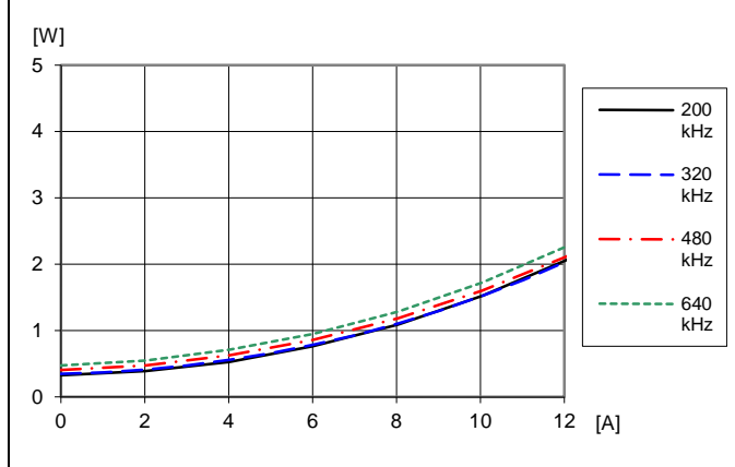
Dissipated power vs. load current and switching frequency at T_{P1} = +25^{\circ}\text{C} . V_I = 12\text{ V} , V_O = 3.3\text{ V} , C_O = 470\ \mu\text{F}/10\ \text{m}\Omega . Default configuration except changed frequency
