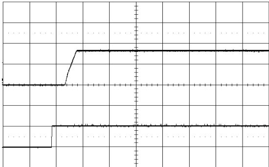
Start-up enabled by connecting V_I at: T_{P1} = +25^\circ\text{C} , V_I = 12\text{ V} , V_O = 3.3\text{ V} C_O = 470\ \mu\text{F}/10\ \text{m}\Omega , I_O = 12\ \text{A} Top trace: output voltage (2 V/div.). Bottom trace: CTRL signal (2 V/div.). Time scale: (20 ms/div.).
