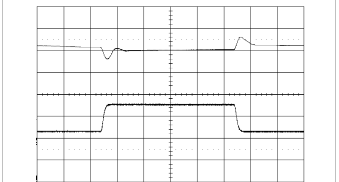
Output voltage response to load current step-change (3-9-3 A) at: T_{P1} = +25^\circ\text{C} , V_i = 12\text{ V} , V_o = 3.3\text{ V} , di/dt=2\text{ A}/\mu\text{s} , f_{sw}=320\text{ kHz} , C_o=470\text{ }\mu\text{F}/10\text{ m}\Omega
