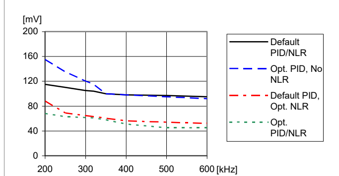
Load transient peak voltage deviation vs. frequency. Step-change (3-9-3 A). T_{P1} = +25^\circ\text{C} . V_i=12\text{ V} , V_o=3.3\text{ V} , C_o=470\text{ }\mu\text{F}/10\text{ m}\Omega
