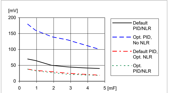
Load transient peak voltage deviation vs. external capacitance. Step-change (3-9-3 A). Parallel coupling of capacitors with 470 \mu\text{F}/10\text{ m}\Omega , T_{P1} = +25^\circ\text{C} . V_i=12\text{ V} , V_o=3.3\text{ V} , f_{sw}=320\text{ kHz} , di/dt=2\text{ A}/\mu\text{s}
