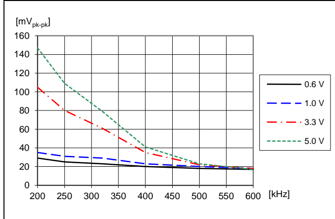
Output voltage ripple V_{pk-pk} at: T_{P1} = +25^{\circ}\text{C} , V_I = 12\text{ V} , C_O = 470\ \mu\text{F}/10\ \text{m}\Omega , I_O = 12\text{ A} resistive load. Default configuration except changed frequency.
