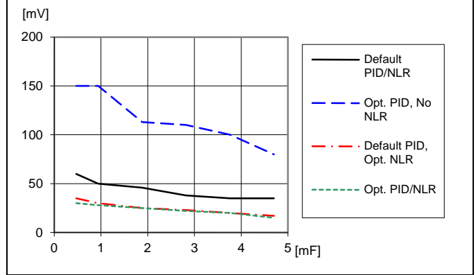
Load transient peak voltage deviation vs. decoupling capacitance. Step-change (3-9-3 A). Parallel coupling of capacitors with 470\ \mu\text{F}/10\ \text{m}\Omega . T_{P1} = +25^{\circ}\text{C} . V_I = 12\text{ V} , V_O = 1.0\text{ V} , f_{sw} = 320\ \text{kHz} , di/dt = 2\ \text{A}/\mu\text{s}
