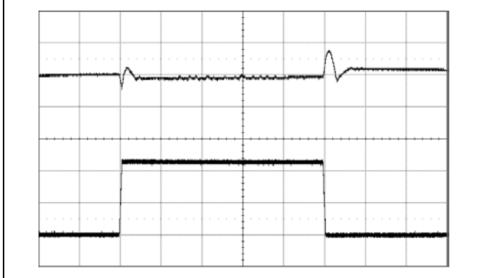
Output voltage response to load current step-change (6.25-18.75-6.25 A) at: T_{P1} = +25^{\circ}\text{C} , V_I = 12\text{ V} , V_O = 1.0\text{ V} di/dt = 2\text{ A}/\mu\text{s} , f_{sw} = 320\text{ kHz} , C_O = 470\ \mu\text{F}/10\text{ m}\Omega Default configuration (DLC and default NLR) Top trace: output voltage (200 mV/div.). Bottom trace: load current (5 A/div.). Time scale: (0.1 ms/div.).
