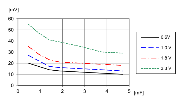
Output voltage ripple V_{pk-pk} at: T_{P1} = +25\text{ }^\circ\text{C} , V_i = 12\text{ V} , I_o = 20\text{ A} . Parallel coupling of capacitors with 470\text{ }\mu\text{F}/10\text{ m}\Omega ,
