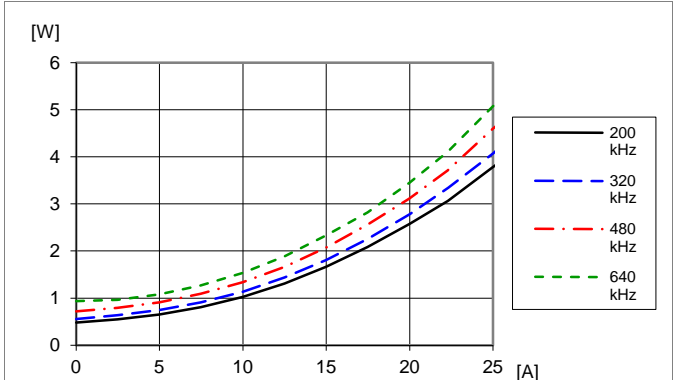
Dissipated power vs. load current and switch frequency at T_{P1} = +25\text{ }^\circ\text{C} , V_I = 12\text{ V} , V_O = 1.0\text{ V} , C_O = 470\text{ }\mu\text{F}/10\text{ m}\Omega . Default configuration except changed frequency
