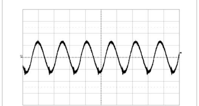
Output voltage ripple at: T_{P1} = +25\text{ }^\circ\text{C} , Trace: output voltage (20 mV/div.). V_i = 12\text{ V} , C_o = 470\text{ }\mu\text{F}/10\text{ m}\Omega Time scale: (2 \mu\text{s}/\text{div.} ). I_o = 20\text{ A}
