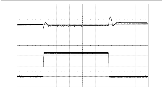
Output voltage response to load current Step-change (6.25-18.75-6.25 A) at: T_{P1} = +25^\circ C , V_I = 12 V , V_O = 1.0 V di/dt = 2 A/\mu s , f_{sw} = 320 kHz C_O = 470 \mu F/10 m\Omega Top trace: output voltage (200 mV/div.). Bottom trace: load current (5 A/div.). Time scale: (0.1 ms/div.).
