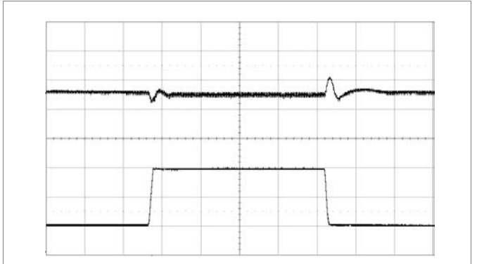
Output voltage response to load current step-change (5-15-5 A) at: T_{P1} = +25\text{ }^\circ\text{C} , V_I = 12\text{ V} , V_O = 1.0\text{ V} , di/dt = 2\text{ A}/\mu\text{s} , f_{sw} = 320\text{ kHz} , C_O = 470\text{ }\mu\text{F}/10\text{ m}\Omega Top trace: output voltage (200 mV/div.). Bottom trace: load current (5 A/div.). Time scale: (0.1 ms/div.).
