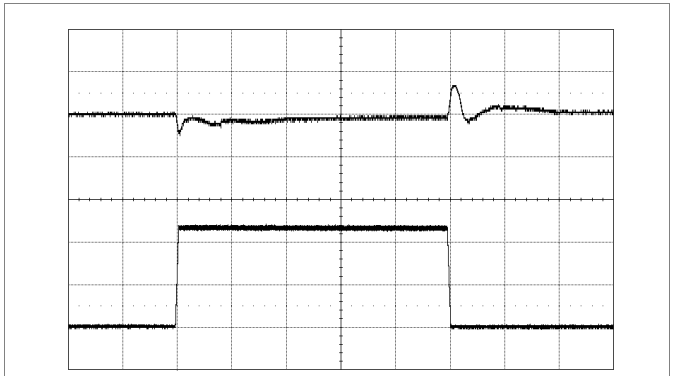
Output voltage response to load Step-change (6.25-18.75-6.25 A) at: Top trace: output voltage (200 mV/div.). T_{P1} = +25^\circ C , V_I = 12 V , V_O = 1.0 V Bottom trace: load current (5 A/div.). di/dt = 2 A/\mu s , f_{sw} = 320 kHz Time scale: (0.1 ms/div.). C_O = 470 \mu F/10 m\Omega
