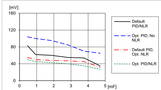
Load transient peak voltage deviation vs. external capacitance. Step-change (5-15-5 A). Parallel coupling of capacitors with 470 \mu\text{F}/10\text{ m}\Omega , T_{P1} = +25\text{ }^\circ\text{C} , V_I = 12\text{ V} , V_O = 1.0\text{ V} , f_{sw} = 320\text{ kHz} , di/dt = 2\text{ A}/\mu\text{s}
