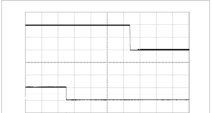
Shut-down enabled by disconnecting V_I at: T_{P1} = +25\text{ }^\circ\text{C} , V_I = 12\text{ V} , V_O = 1.0\text{ V} C_O = 470\text{ }\mu\text{F}/10\text{ m}\Omega , I_O = 20\text{ A} Top trace: output voltage (0.5 V/div.). Bottom trace: CTRL signal (5 V/div.). Time scale: (2 ms/div.).
