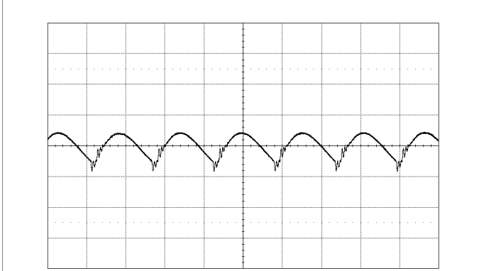
Output voltage ripple at: T_{P1} = +25\text{ }^\circ\text{C} , Trace: output voltage (20 mV/div.). V_i = 12\text{ V} , C_o = 470\text{ }\mu\text{F}/10\text{ m}\Omega Time scale: (2 \mu\text{s}/\text{div.} ). I_o = 25\text{ A}
