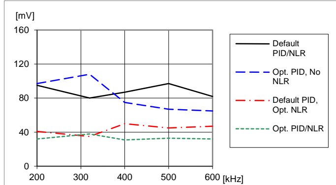
Load transient peak voltage deviation vs. frequency. Step-change (5-15-5 A). T_{P1} = +25\text{ }^\circ\text{C} , V_I = 12\text{ V} , V_O = 1.0\text{ V} , C_O = 470\text{ }\mu\text{F}/10\text{ m}\Omega
