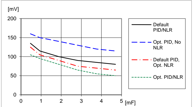
Load transient peak voltage deviation vs. external capacitance. Step-change (5-15-5 A). Parallel coupling of capacitors with 470 \mu F /10 m \Omega , T_{P1} = +25^\circ C , V_I = 12 V , V_O = 3.3 V , f_{sw} = 320 kHz , di/dt = 2 A/\mu s
