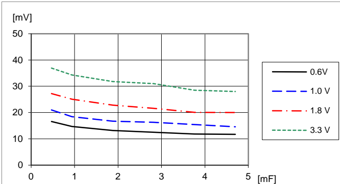
Output voltage ripple V_{pk-pk} at: T_{P1} = +25\text{ }^\circ\text{C} , V_i = 12\text{ V} , I_o = 25\text{ A} . Parallel coupling of capacitors with 470 \mu\text{F}/10\text{ m}\Omega
