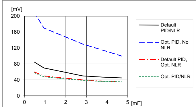
Load transient peak voltage deviation vs. external capacitance. Step-change (5-15-5 A). Parallel coupling of capacitors with 470 \mu F /10 m \Omega , T_{P1} = +25^\circ C , V_I = 12 V , V_O = 1.0 V , f_{sw} = 320 kHz , di/dt = 2 A/\mu s
