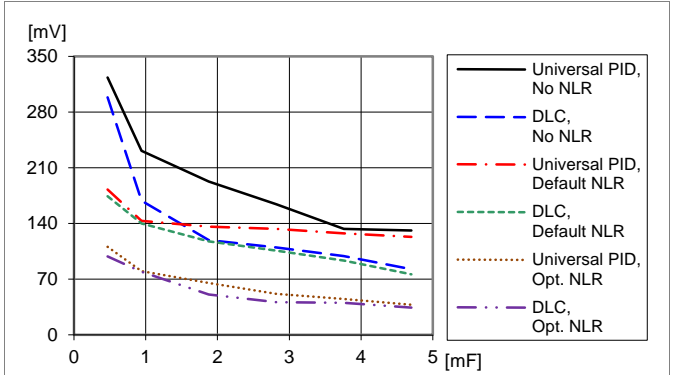
Load transient peak voltage deviation vs. external capacitance. Step (6.25-18.75-6.25 A). Parallel coupling of capacitors with 470 \mu F/10 m\Omega , T_{P1} = +25^\circ C . V_I = 12 V , V_O = 3.3 V , f_{sw} = 320 kHz , di/dt = 2 A/\mu s
