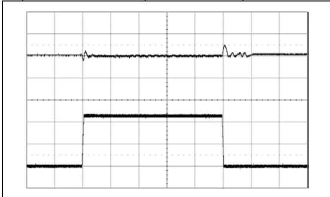
Output voltage response to load current step-change (6.25-18.75-6.25 A) at: T_{P1} = +25^{\circ}\text{C} , V_I = 12\text{ V} , V_O = 1.0\text{ V} di/dt = 2\text{ A}/\mu\text{s} , f_{sw} = 320\text{ kHz} , C_O = 470\ \mu\text{F}/10\text{ m}\Omega Top trace: output voltage (200 mV/div.). Bottom trace: load current (5 A/div.). Time scale: (0.1 ms/div.).
