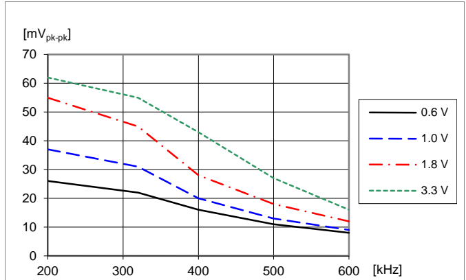
Output voltage ripple V_{pk-pk} at: T_{P1} = +25\text{ }^\circ\text{C} , V_i = 12\text{ V} , C_o = 470\text{ }\mu\text{F}/10\text{ m}\Omega , I_o = 20\text{ A} . Default configuration except changed frequency.
