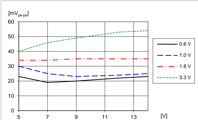
Output voltage ripple V_{pk-pk} at: T_{P1} = +25\text{ }^\circ\text{C} , C_o = 470\text{ }\mu\text{F}/10\text{ m}\Omega , I_o = 20\text{ A} .
