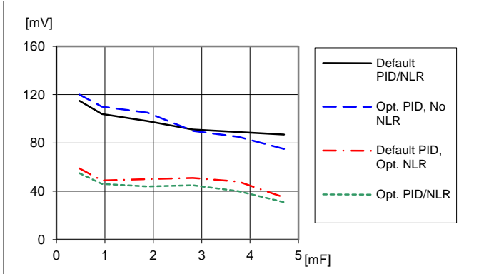
Load transient peak voltage deviation vs. external capacitance. Step-change (5-15-5 A). Parallel coupling of capacitors with 470 \mu\text{F}/10\text{ m}\Omega , T_{P1} = +25\text{ }^\circ\text{C} , V_I = 12\text{ V} , V_O = 3.3\text{ V} , f_{sw} = 320\text{ kHz} , di/dt = 2\text{ A}/\mu\text{s}
