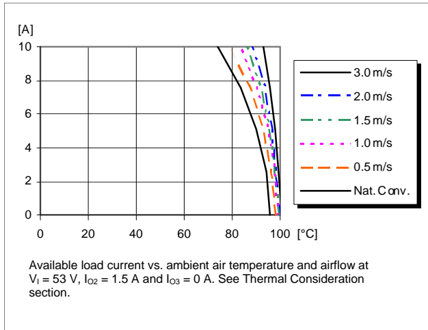
Output Current Derating, Basic Insulation (P*)
