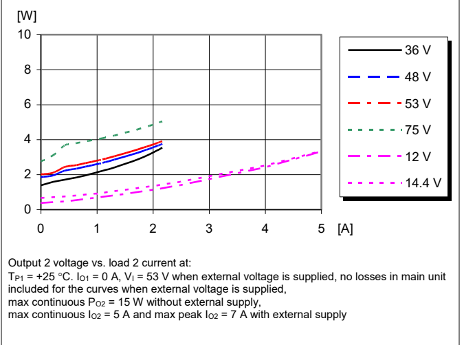
Power Dissipation, unadjusted output voltage
