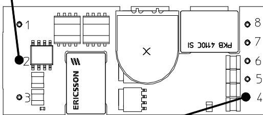
Pin 2 for measurement of maximum peak product reflow temperature, T_p
