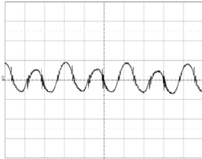
Output voltage ripple at: T_{P1} = +25^\circ\text{C} , V_i = 53\text{ V} , I_o = 20\text{ A} resistive load. Trace: output voltage (20 mV/div.). Time scale: (2 \mu\text{s} /div.).
