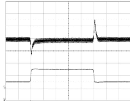
Output voltage response to load current step-change (5-15 A) at: T_{P1} = +25^\circ\text{C} , V_i = 53\text{ V} . Top trace: output voltage (200 mV/div.). Bottom trace: load current (10 A/div.). Time scale: (0.1 ms/div.).
