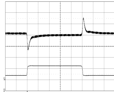
Output voltage response to load current step- change (3.75-11.25-3.75 A) at: T_{ref} = +25^\circ\text{C} , V_i = 53\text{ V} . Top trace: output voltage (200 mV/div.). Bottom trace: load current (10 A/div.). Time scale: (0.1 ms/div.).
