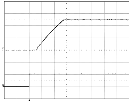
Start-up enabled by connecting V_1 at: T_{ref} = +25^{\circ}\text{C} , V_1 = 53\text{ V} , I_O = 25\text{ A} resistive load. Top trace: output voltage (2 V/div.). Bottom trace: input voltage (50 V/div.). Time scale: (5 ms/div.).
