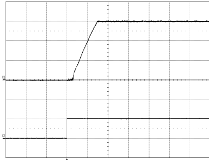
Start-up enabled by connecting V_i at: T_{ref} = +25^{\circ}\text{C} , V_i = 53\text{ V} , I_O = 30\text{ A} resistive load. Top trace: output voltage (0.5 V/div.). Bottom trace: input voltage (20 V/div.). Time scale: (5 ms/div.).
