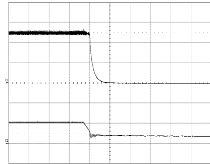
Shut-down enabled by disconnecting V_1 at: T_{ref} = +25^{\circ}\text{C} , V_1 = 53\text{ V} , I_O = 25\text{ A} resistive load. Top trace: output voltage (2 V/div.). Bottom trace: input voltage (50 V/div.). Time scale: (0.2 ms/div.).
