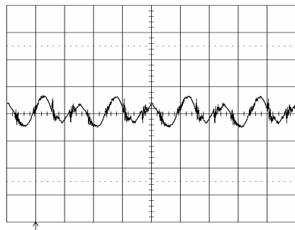
Output voltage ripple at: T_{ref} = +25^{\circ}\text{C} , V_1 = 53\text{ V} , I_O = 25\text{ A} resistive load. Trace: output voltage (20 mV/div.). Time scale: (2 \mu\text{s} /div.).
