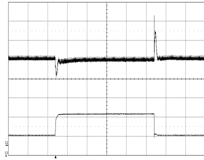
Output voltage response to load current step-change (6.25-18.75-6.25 A) at: T_{ref} = +25^{\circ}\text{C} , V_1 = 53\text{ V} . Top trace: output voltage (200 mV/div.). Bottom trace: load current (10 A/div.). Time scale: (0.1 ms/div.).
