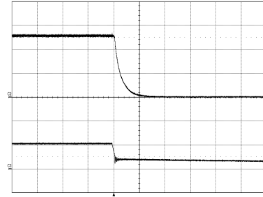
Shut-down enabled by disconnecting V_i at: T_{ref} = +25^{\circ}\text{C} , V_i = 53\text{ V} , I_o = 15\text{ A} resistive load. Top trace: output voltage (2 V/div.). Bottom trace: input voltage (50 V/div.). Time scale: (0.2 ms/div.).
