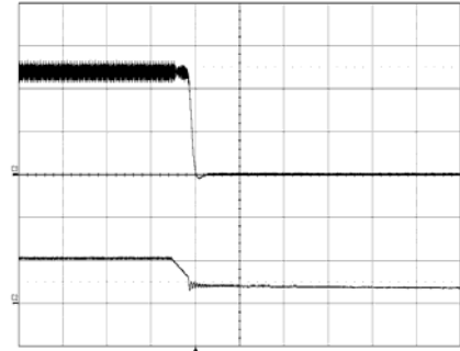
Shut-down enabled by disconnecting V_i at: T_{ref} = +25^\circ\text{C} , V_i = 53\text{ V} , I_o = 30\text{ A} resistive load. Top trace: output voltage (0.5 V/div.). Bottom trace: input voltage (50 V/div.). Time scale: (0.1 ms/div.).
