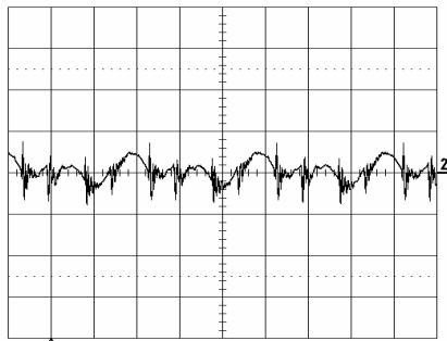
Output voltage ripple at: T_{ref} = +25^\circ\text{C} , V_i = 53\text{ V} , I_o = 30\text{ A} resistive load. Trace: output voltage (20 mV/div.). Time scale: (2 \mu\text{s} /div.).
