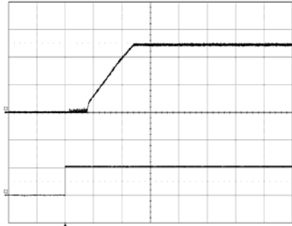
Start-up enabled by connecting V_i at: T_{ref} = +25^\circ\text{C} , V_i = 53\text{ V} , I_o = 30\text{ A} resistive load. Top trace: output voltage (0.5 V/div.). Bottom trace: input voltage (50 V/div.). Time scale: (5 ms/div.).
