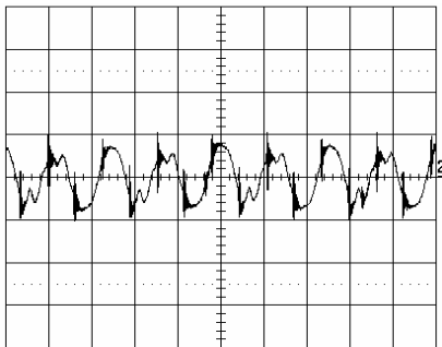
Output voltage ripple at: T_{ref} = +25^{\circ}\text{C} , V_i = 53\text{ V} , I_o = 15\text{ A} resistive load. Trace: output voltage (20 mV/div.). Time scale: (2 μs/div.).
