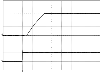
Start-up enabled by connecting V_i at: T_{ref} = +25^{\circ}\text{C} , V_i = 53\text{ V} , I_o = 15\text{ A} resistive load. Top trace: output voltage (2 V/div.). Bottom trace: input voltage (50 V/div.). Time scale: (5 ms/div.).
