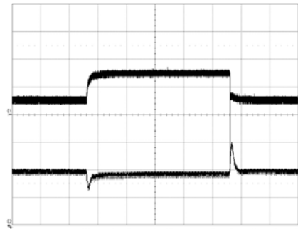
Output voltage response to load current step-change (5.5-17.5-5.5 A) at: T_{ref} = +25^\circ\text{C} , V_i = 53\text{ V} . Top trace: output voltage (200 mV/div.). Bottom trace: load current (10 A/div.). Time scale: (0.1 ms/div.).
