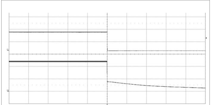
Output disabled by removing V_I at: T_{P1} = +25^\circ\text{C} , V_I = 24\text{ V} , I_O = 2\text{ A} resistive load. Top trace: output voltage (10 V/div). Bottom trace: input voltage (10 V/div). Time scale: (200 ms/div).
