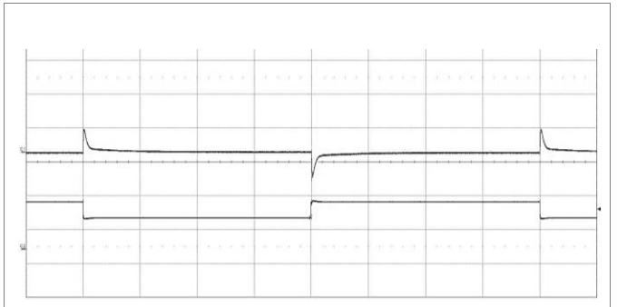
Output voltage response to load current step-change (1.0-1.5-1.0 A) at: T_{P1} = +25^\circ\text{C} , V_I = 24\text{ V} . Top trace: output voltage (500 mV/div). Bottom trace: load current (1 A/div). Time scale: (2 ms/div).
