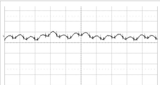
Output voltage ripple at: T_{P1} = +25^\circ\text{C} , V_I = 24\text{ V} , I_O = 2.5\text{ A} resistive load. Trace: output voltage (20 mV/div.). Time scale: (5 \mu\text{s} /div.). 20 MHz bandwidth
