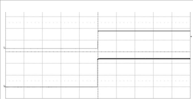
Start-up enabled by connecting V_I at: T_{P1} = +25^\circ\text{C} , V_I = 24\text{ V} , I_O = 2\text{ A} resistive load. Top trace: output voltage (10 V/div). Bottom trace: input voltage (10 V/div). Time scale: (200 ms/div).
