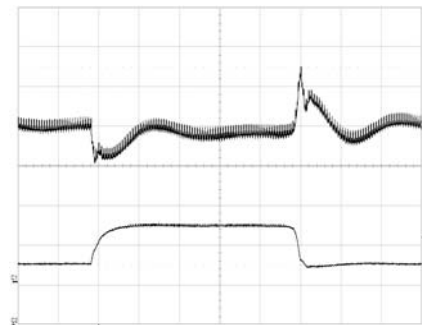
Output voltage response to load current step-change (25-75-25 A) at: T_{P1} = +25^{\circ}\text{C} , V_i = 53\text{ V} .
