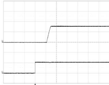
Start-up enabled by connecting V_i at: T_{P1} = +25^{\circ}\text{C} , V_i = 53\text{ V} , I_o = 100\text{ A} resistive load.
