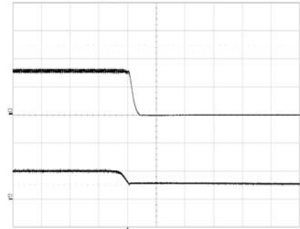
Shut-down enabled by disconnecting V_i at: T_{P1} = +25^{\circ}\text{C} , V_i = 53\text{ V} , I_o = 100\text{ A} resistive load.
