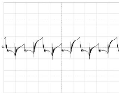
Output voltage ripple at: T_{P1} = +25^{\circ}\text{C} , V_i = 53\text{ V} , I_o = 100\text{ A} resistive load.
