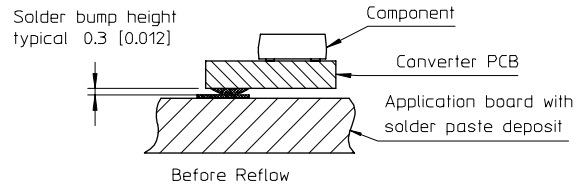
APPLICATION VIEW (detail)
