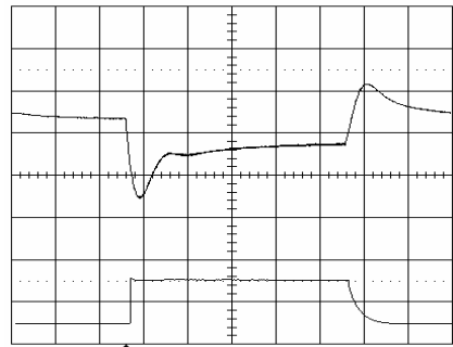
Output voltage response to load current step-change (0.25-0.75-0.25 A) at: T_{ref} = +25^{\circ}\text{C} , V_i = 27\text{ V} .
