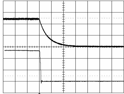
Shut-down enabled by disconnecting V_i at: T_{ref} = +25^{\circ}\text{C} , V_i = 27\text{ V} , I_o = 1\text{ A} resistive load.
