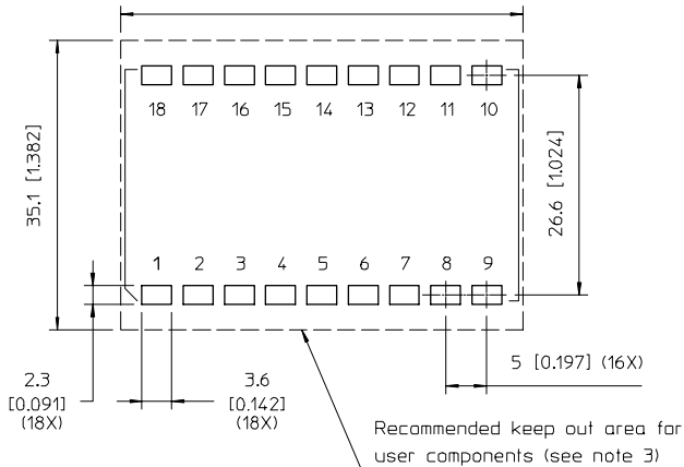
FOOTPRINT (top view, application board) 48.8 [1.921]
