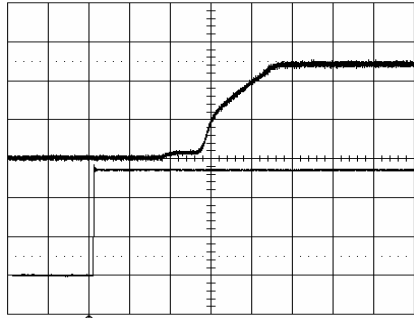
Start-up enabled by connecting V_i at: T_{ref} = +25^{\circ}\text{C} , V_i = 27\text{ V} , I_o = 1\text{ A} resistive load.
