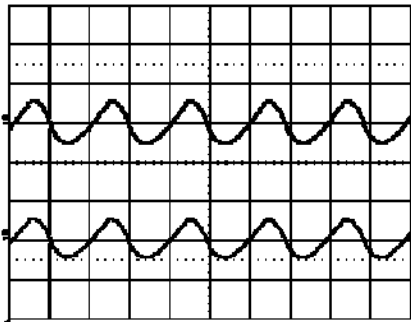
Output voltage ripple at: T_{ref} = +25^\circ\text{C} , V_i = 53\text{ V} , I_{o1} = 0.62\text{ A} , I_{o2} = 0.62\text{ A} resistive load. Top trace: output voltage 1 (20 mV/div). Bottom trace: output voltage 2 (20 mV/div). Time scale: (1 μs/div.).
