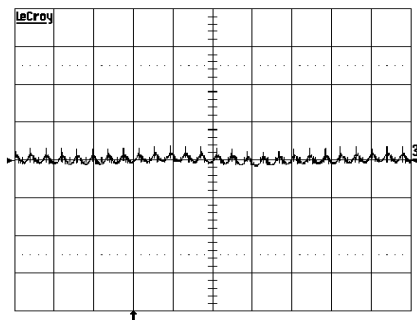
Output voltage ripple at: T_{ref} = +25^{\circ}C , V_i = 53 V , I_o = 1.2 A resistive load. Trace: output voltage (10 mV/div.). Time scale: (5 \mu s/div.).
