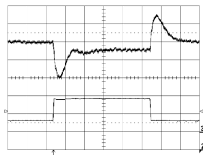
Output voltage response to load current step-change (0.3-0.9-0.3 A) at: T_{ref} = +25^{\circ}C , V_i = 53 V . Top trace: output voltage (100 mV/div.). Bottom trace: load current (0.5 A/div.). Time scale: (0.1 ms/div.).
