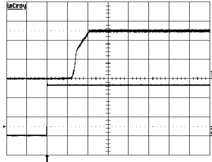
Start-up enabled by connecting V_i at: T_{ref} = +25^{\circ}C , V_i = 53 V , I_o = 1.2 A resistive load. Top trace: output voltage (2.0 V/div.). Bottom trace: input voltage (20 V/div.). Time scale: (2 ms/div.).
