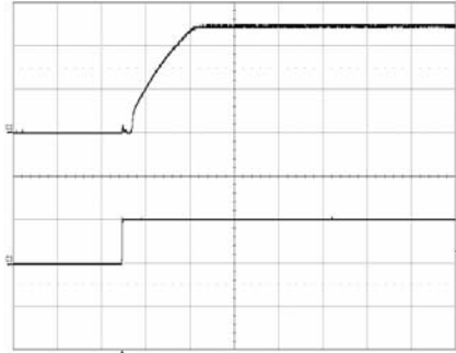
Start-up enabled by connecting V_i at: T_{P1} = +25^\circ\text{C} , V_i = 53\text{ V} , I_o = 7\text{ A} load.
