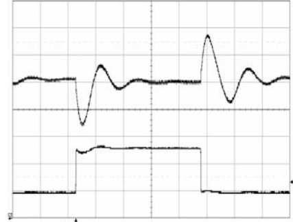
Output voltage response to load current step- change (1.75 - 5.25 - 1.75 A) at: T_{P1} = +25^\circ\text{C} , V_i = 53\text{ V} , C_o = 690\mu\text{F}
