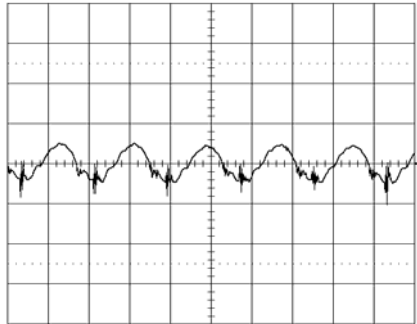
Output voltage ripple at: T_{P1} = +25^\circ\text{C} , V_i = 53\text{ V} , I_o = 7\text{ A} resistive load.
