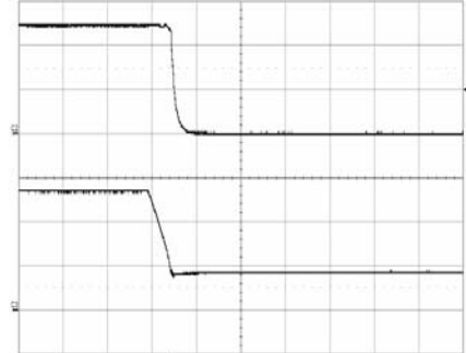
Shut-down enabled by disconnecting V_i at: T_{P1} = +25^\circ\text{C} , V_i = 53\text{ V} , I_o = 7\text{ A} resistive load.
