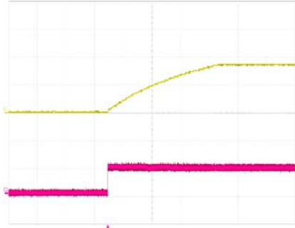
Start-up enabled by connecting V_I at: T_{ref} = +25^\circ\text{C} , I_O = 2.25\text{ A} resistive load, V_I = 5.0\text{ V} .
