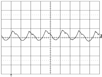
Output voltage ripple (5 mV/div.) at: T_{ref} = +25^\circ\text{C} , I_O = 2.25\text{ A} resistive load, V_I = 5.0\text{ V} . Time scale: 2 \mu\text{s} /div.
