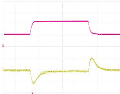
Output voltage response to load current step- change (1.125-2.25-1.125 A) at: T_{ref} = +25^\circ\text{C} , V_I = 5.0\text{ V} .
