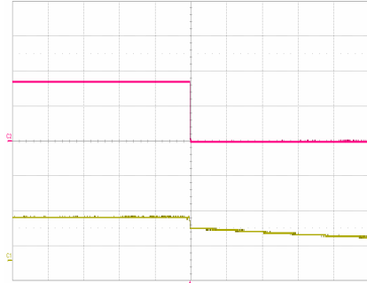
Shut-down enabled by disconnecting V_I at: T_{ref} = +25^\circ\text{C} , I_O = 2.25\text{ A} resistive load, V_I = 5.0\text{ V} .
