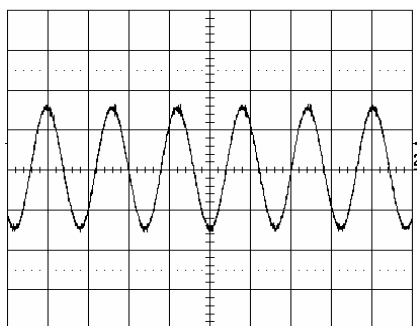
Output voltage ripple (20mV/div.) at: T_{ref} = +25^\circ\text{C} , I_O = 6\text{ A} resistive load, V_i = 12.0\text{ V} . Time scale: 2 µs/div. See the filter in the Output ripple and noise section (EMC Specification).
