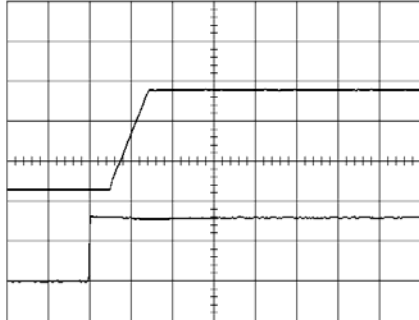
Start-up enabled by connecting V_i at: T_{ref} = +25^\circ\text{C} , I_O = 10\text{ A} resistive load, V_i = 3.3\text{ V} . Top trace: output voltage (1.0 V/div.). Bottom trace: input voltage (2 V/div.). Time scale: 5 ms/div..
