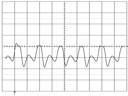
Output voltage ripple (20mV/div.) at: T_{ref} = +25^\circ\text{C} , I_O = 10\text{ A} resistive load, V_I = 5.0\text{ V} . Time scale: 2 \mu\text{s}/\text{div} . See the filter in the Output ripple and noise section (EMC Specification).
