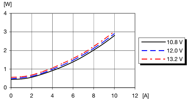
Dissipated power vs. load current and input voltage at T_{ref} = +25^{\circ}C
