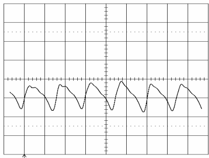
Output voltage ripple (20mV/div.) at: T_{ref} = +25^\circ\text{C} , I_O = 12\text{ A} resistive load, V_I = 12.0\text{ V} . Time scale: 2 \mu\text{s} /div See the filter in the Output ripple and noise section (EMC Specification).
