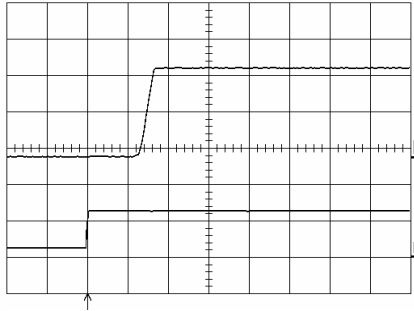
Start-up enabled by connecting V_I at: T_{ref} = +25^\circ\text{C} , I_O = 12\text{ A} resistive load, V_I = 12.0\text{ V} . Top trace: output voltage (1.0 V/div.). Bottom trace: input voltage (10 V/div.). Time scale: 10 ms/div.
