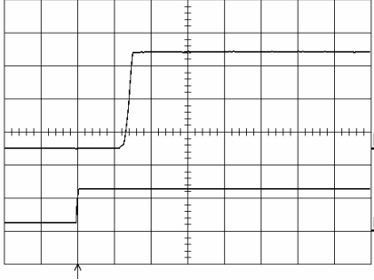
Start-up enabled by connecting V_I at: T_{ref} = +25^\circ\text{C} , I_O = 12\text{ A} resistive load, V_I = 12.0\text{ V} . Top trace: output voltage (0.5 V/div.). Bottom trace: input voltage (10 V/div.). Time scale: 10 ms/div.
