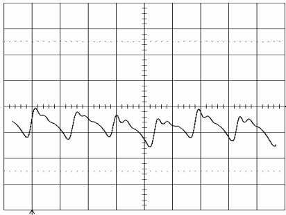
Output voltage ripple (20mV/div.) at: T_{ref} = +25^\circ\text{C} , I_O = 12\text{ A} resistive load, V_I = 12.0\text{ V} . Time scale: 2 μs/div. See the filter in the Output ripple and noise section (EMC Specification).
