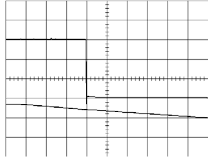
Shut-down enabled by disconnecting V_I at: T_{ref} = +25^\circ\text{C} , I_O = 12\text{ A} resistive load, V_I = 12.0\text{ V} . Top trace: output voltage (0.5 V/div.). Bottom trace: input voltage (10 V/div.). Time scale: 5.0 ms/div.
