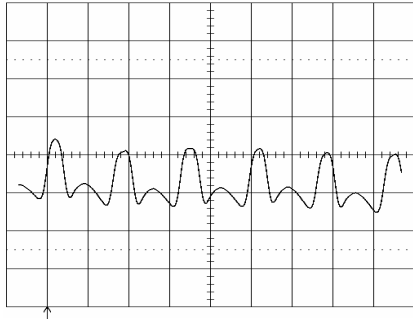
Output voltage ripple (20mV/div.) at: T_{ref} = +25^\circ\text{C} , I_O = 22\text{ A} resistive load, V_i = 5.0\text{ V} . Time scale: 2 \mu\text{s} /div. See the filter in the Output ripple and noise section (EMC Specification).
