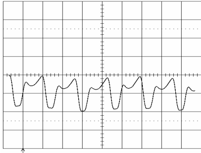
Output voltage ripple (20mV/div.) at: T_{ref} = +25^\circ\text{C} , I_o = 22\text{ A} resistive load, V_i = 5.0\text{ V} . Time scale: 2 μs/div. See the filter in the Output ripple and noise section (EMC Specification).
