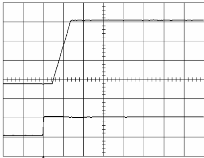
S Start-up enabled by connecting V_i at: T_{ref} = +25^\circ\text{C} , I_o = 22\text{ A} resistive load, V_i = 5.0\text{ V} .. Top trace: output voltage (1.0 V/div.). Bottom trace: input voltage (5 V/div.). Time scale: 5 ms/div..
