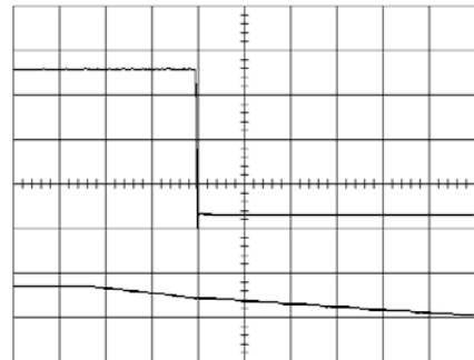
Shut-down enabled by disconnecting V_i at: T_{ref} = +25^\circ\text{C} , I_O = 18\text{ A} resistive load, V_i = 12.0\text{ V} . Top trace: output voltage (1.0 V/div.). Bottom trace: input voltage (10 V/div.). Time scale: 5.0 ms/div.
