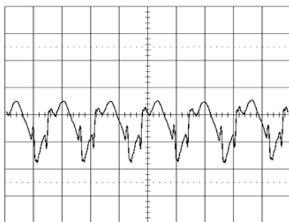
Output voltage ripple (20mV/div.) at: T_{ref} = +25^\circ\text{C} , I_O = 18\text{ A} resistive load, V_i = 12.0\text{ V} . Time scale: 2 \mu\text{s} /div. See the filter in the Output ripple and noise section (EMC Specification).
