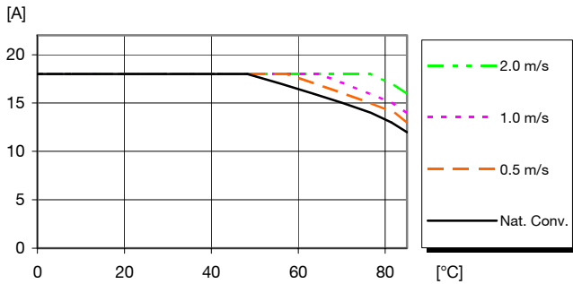
Available load current vs. ambient air temperature and airflow at V_I = 12.0 V, V_{OUT} = 1.8 V . See Thermal Consideration section.
