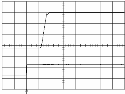
Start-up enabled by connecting V_i at: T_{ref} = +25^\circ\text{C} , I_O = 18\text{ A} resistive load, V_i = 12.0\text{ V} . Top trace: output voltage (1.0 V/div.). Bottom trace: input voltage (10 V/div.). Time scale: 10 ms/div.
