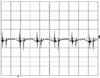
Output voltage ripple (20mV/div.) at: T_{ref} = +25^{\circ}\text{C} , I_O = 26\text{ A} resistive load, V_i = 12.0\text{ V} . Time scale: 1 \mu\text{s} /div. See the filter in the Output ripple and noise section (EMC Specification).
