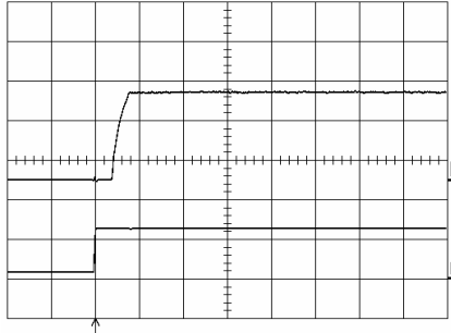
Start-up enabled by connecting V_i at: T_{ref} = +25^{\circ}\text{C} , I_O = 26\text{ A} resistive load, V_i = 12.0\text{ V} . Top trace: output voltage (0.5 V/div.). Bottom trace: input voltage (10 V/div.). Time scale: 10 ms/div.
