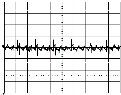
Output voltage ripple (20 mV/div.) at: T_{ref} = +25^\circ\text{C} , I_o = 50\text{ A} resistive load, V_i = 12.0\text{ V} . Time scale: 2 \mu\text{s} /div. See the filter in the Output ripple and noise section (EMC Specification).
