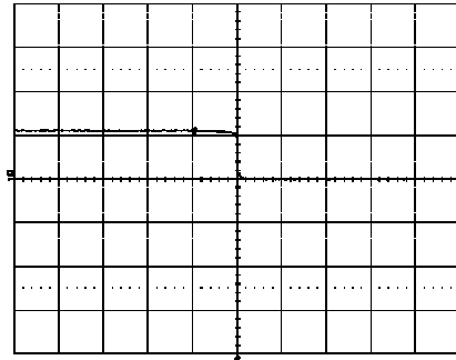
Shut-down enabled by disconnecting V_i at: T_{ref} = +25^\circ\text{C} , I_o = 50\text{ A} resistive load, V_i = 12.0\text{ V} . Top trace: output voltage (1.0 V/div.). Time scale: 1.0 ms/div.
