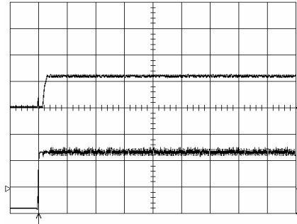
Start-up enabled by connecting V_i at: T_{ref} = +25^\circ\text{C} , I_o = 50\text{ A} resistive load, V_i = 12.0\text{ V} . Top trace: output voltage (1.0 V/div.). Bottom trace: input voltage (5 V/div.). Time scale: 20 ms/div.
