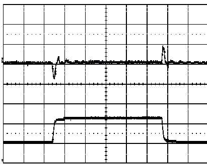
Output voltage response to load current step- change (25-50-25 A) at: T_{ref} = +25^\circ\text{C} , V_i = 12.0\text{ V} . Top trace: output voltage (100 mV/div.). Bottom trace: load current (20 A/div.). Time scale: 0.2 ms/div.
