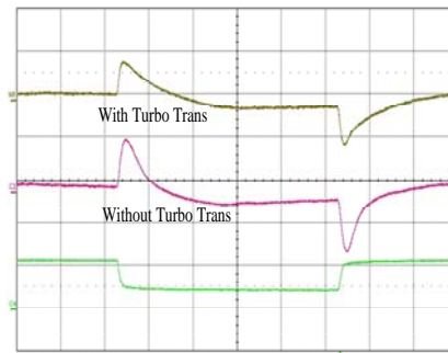
Output voltage response to load current step- change (7.5-22.5-7.5 A) at: T_{ref} = +25^{\circ}C , V_i = 5 V . Top trace: output voltage (100 mV/div.). Middle trace: output voltage (100mV/div.). Bottom trace: load current (20 A/div.). Time scale: (0.1 ms/div.).
