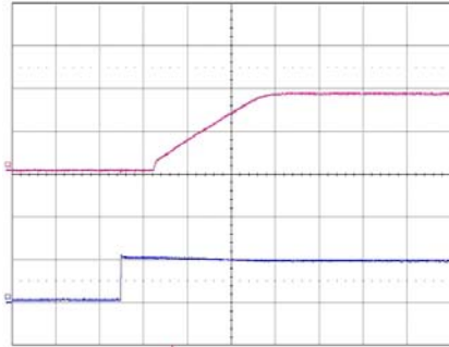
Start-up enabled by connecting V_i at: T_{ref} = +25^{\circ}C , V_i = 5 V , I_O = 30 A resistive load. Top trace: output voltage (1 V/div.). Bottom trace: input voltage (5 V/div.). Time scale: (5 ms/div.).
