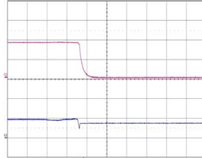
Shut-down enabled by disconnecting V_i at: T_{ref} = +25^{\circ}C , V_i = 5 V , I_O = 30 A resistive load. Top trace: output voltage (1 V/div.). Bottom trace: input voltage (5 V/div.). Time scale: (0.5 ms/div.).
