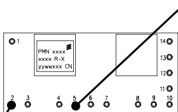
Pin 5 for measurement of minimum solder joint temperature, T_{PIN}
