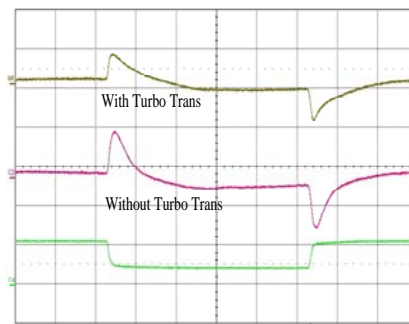
Output voltage response to load current step- change (7.5-22.5-7.5 A) at: T_{ref} = +25^{\circ}\text{C} , V_i = 5\text{ V} . Top trace: output voltage (100 mV/div.). Middle trace: output voltage (100mV/div.). Bottom trace: load current (20 A/div.). Time scale: (0.1 ms/div.).
