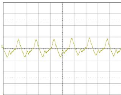
Output voltage ripple at: T_{ref} = +25^{\circ}\text{C} , V_i = 5\text{ V} , I_O = 30\text{ A} resistive load. Trace: output voltage (2 mV/div.). Time scale: (2 μs/div.).
