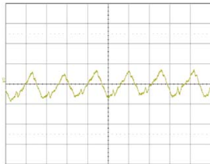
Output voltage ripple at: T_{ref} = +25^{\circ}C , V_i = 5 V , I_O = 30 A resistive load. Trace: output voltage (2 mV/div.). Time scale: (2 μs/div.).
