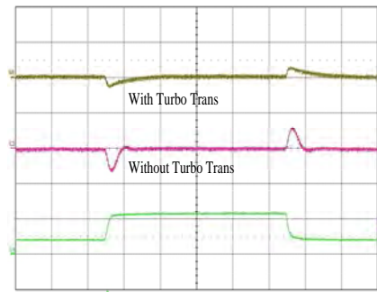
Output voltage response to load current step-change (4-12-4 A) at: T_{ref} = +25^{\circ}C, V_I = 5 V. Top trace: output voltage (100 mV/div). Middle trace: output voltage (100 mV/div). Bottom trace: load current (10 A/div).
