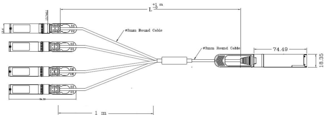
Figure 7. Mechanical Outline
