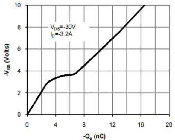
Figure 6: Gate-Charge Characteristics
