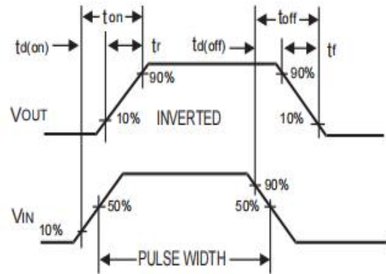
Figure 10: Switching Waveform
