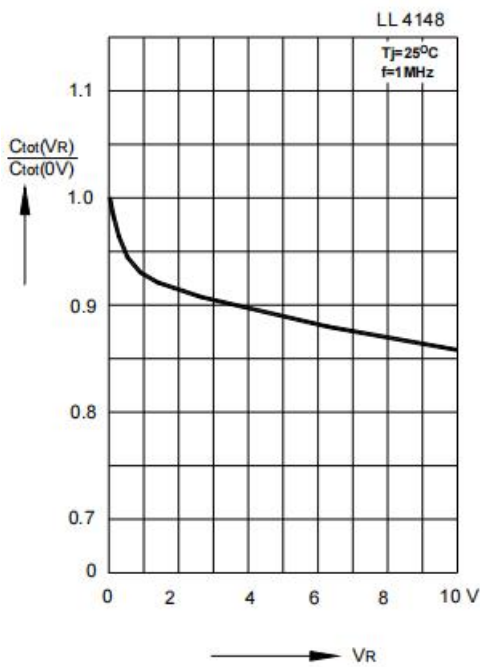
Figure 3: Capacitance Characteristics
