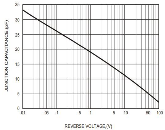
Figure 4: Junction Capacitance
