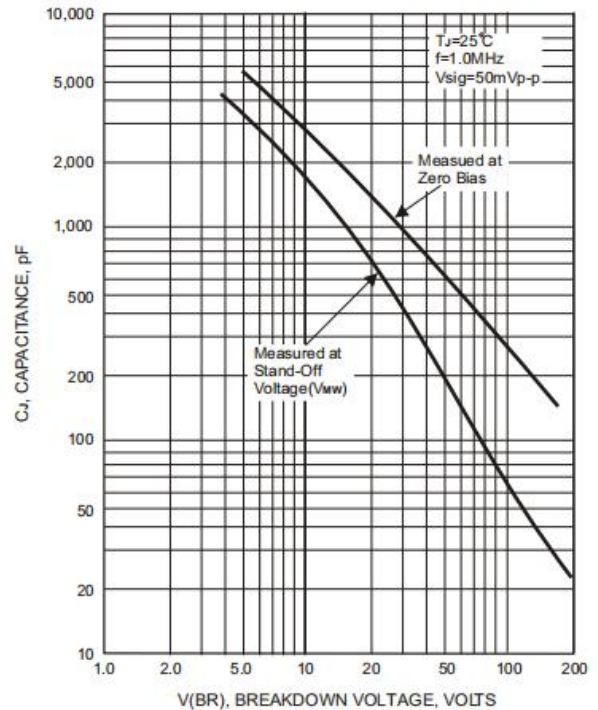
FIG.4-TYPICAL JUNCTION CAPACITANCE
