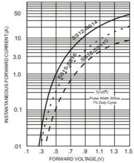
FIG.2-TYPICAL FORWARD CHARACTERISTICS
