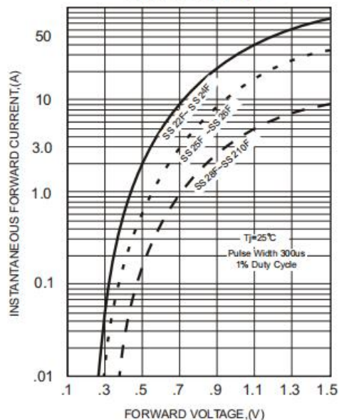
FIG.2-TYPICAL FORWARD CHARACTERISTICS
