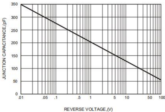
FIG.4-TYPICAL JUNCTION CAPACITANCE
