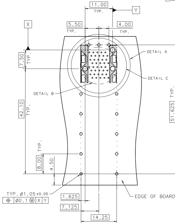
RECOMMENDED HOST BOARD LAYOUT
