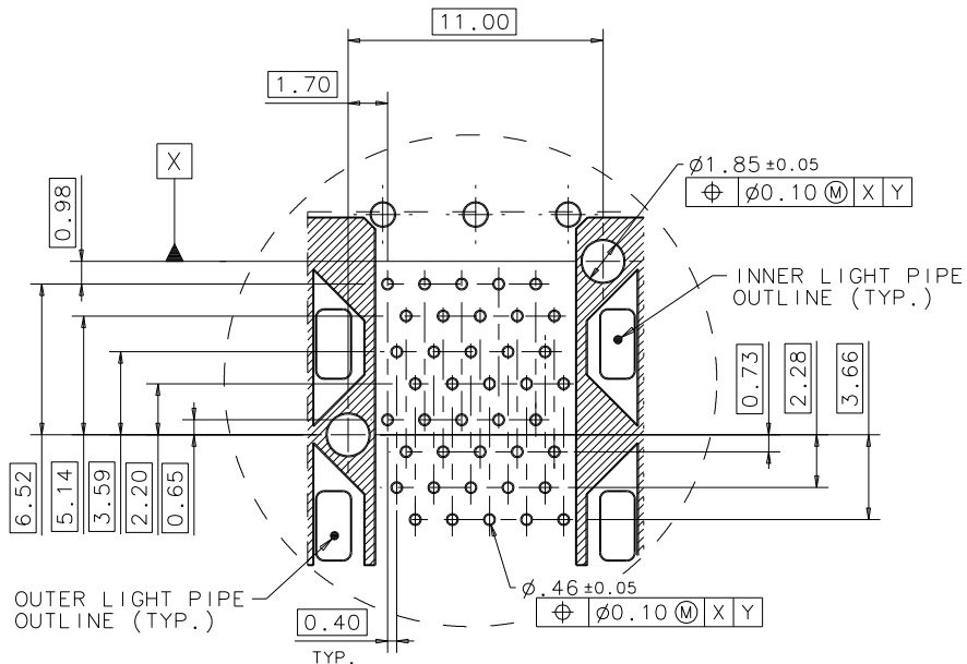
DETAIL A
