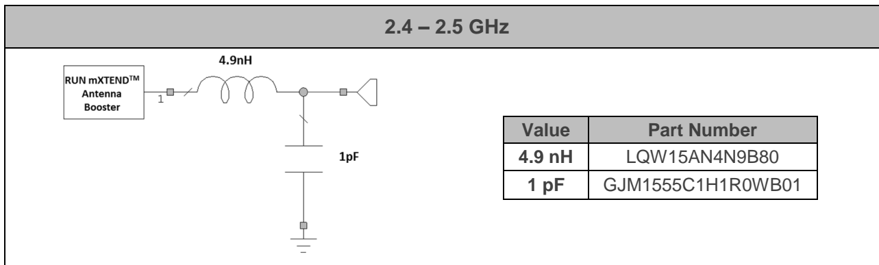
Figure 5 – Matching Network implemented in the evaluation board (Figure 4).
