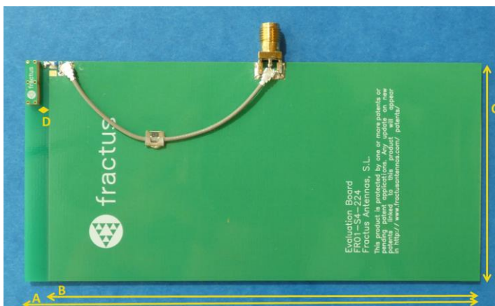
Figure 1 – EB_FR01-S4-224-2400. Evaluation Board providing operation from 2.4 GHz to 2.5 GHz.
