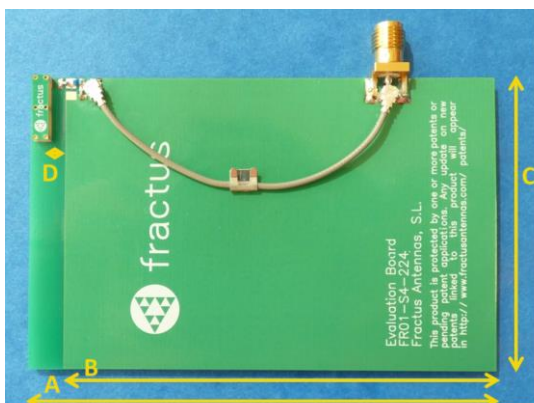
Figure 4 – EB_FR01-S4-224-CR80-2400 in CR80 standard format. Evaluation Board providing operation from 2.4 GHz to 2.5 GHz.
