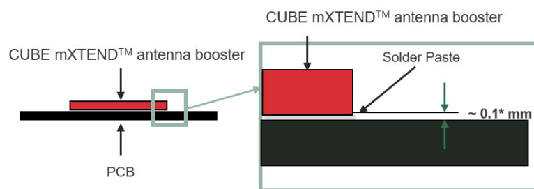
Figure 7 – Soldering Details.
