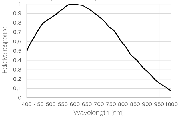
FSM-IMX296C (Color):
