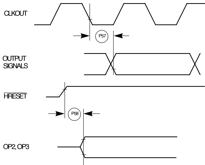
Figure 26. PCMCIA Output Port Timing Diagram
