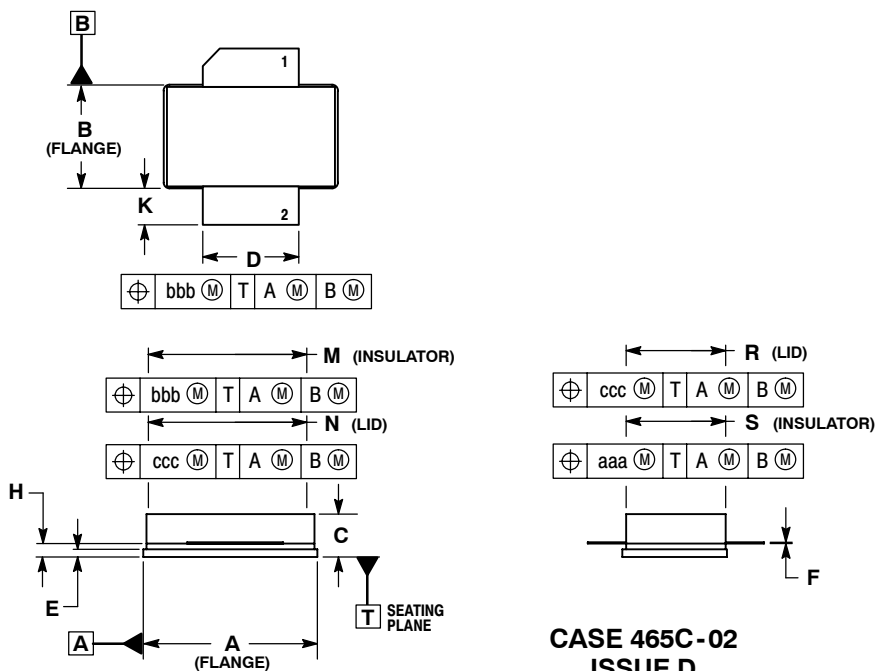
CASE 465B-03 ISSUE D NI-880 MRFE6S9205HR3
