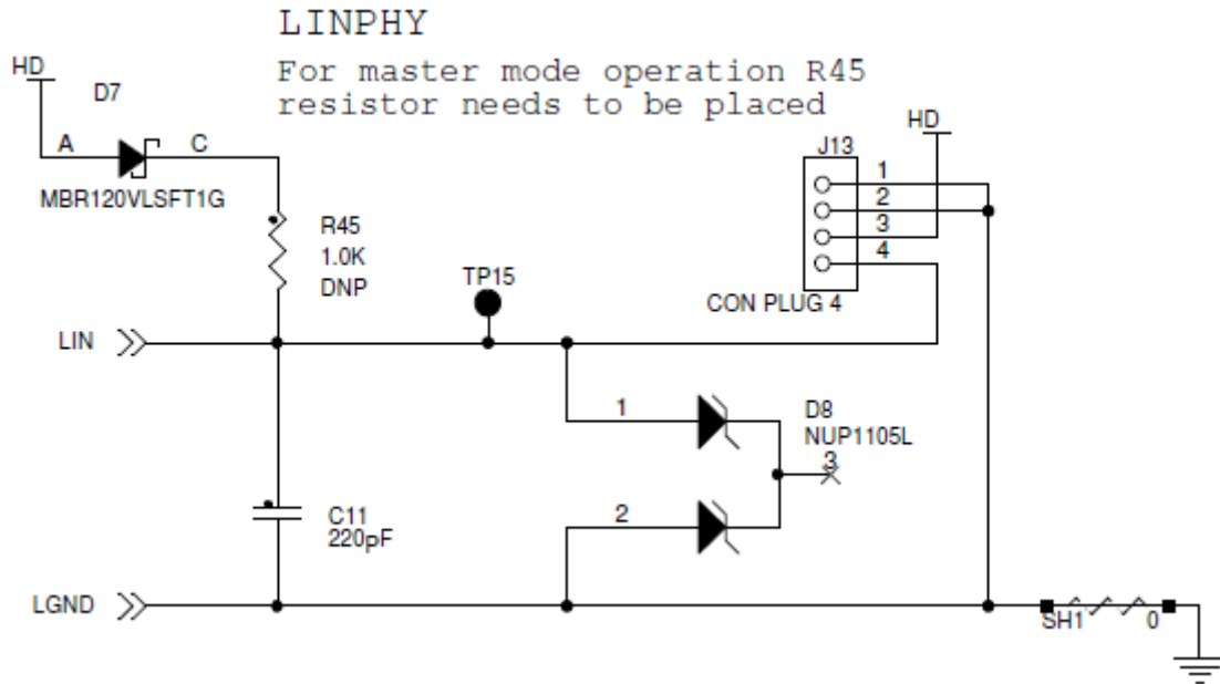
Figure 7. LIN interface
