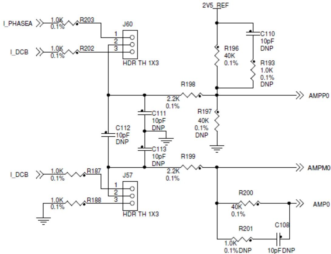
Figure 12. Phase A/DCB Bus current sense option
