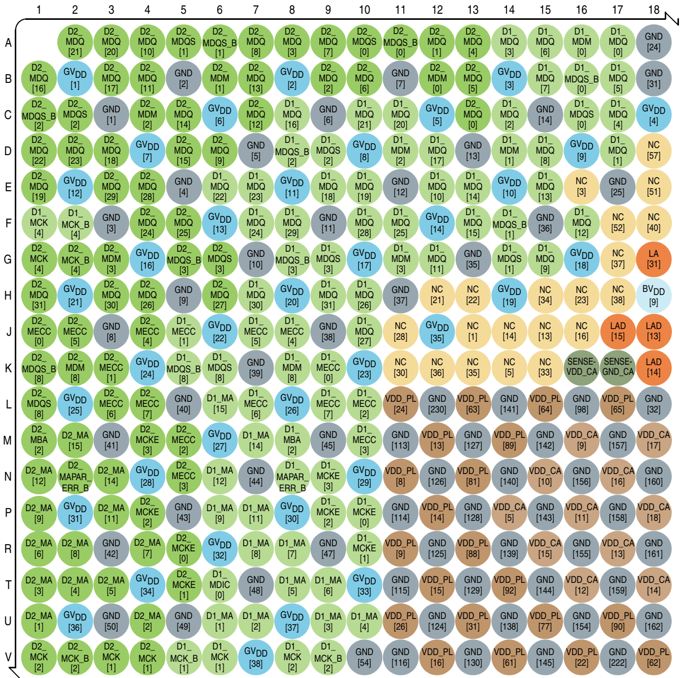
DETAIL A
