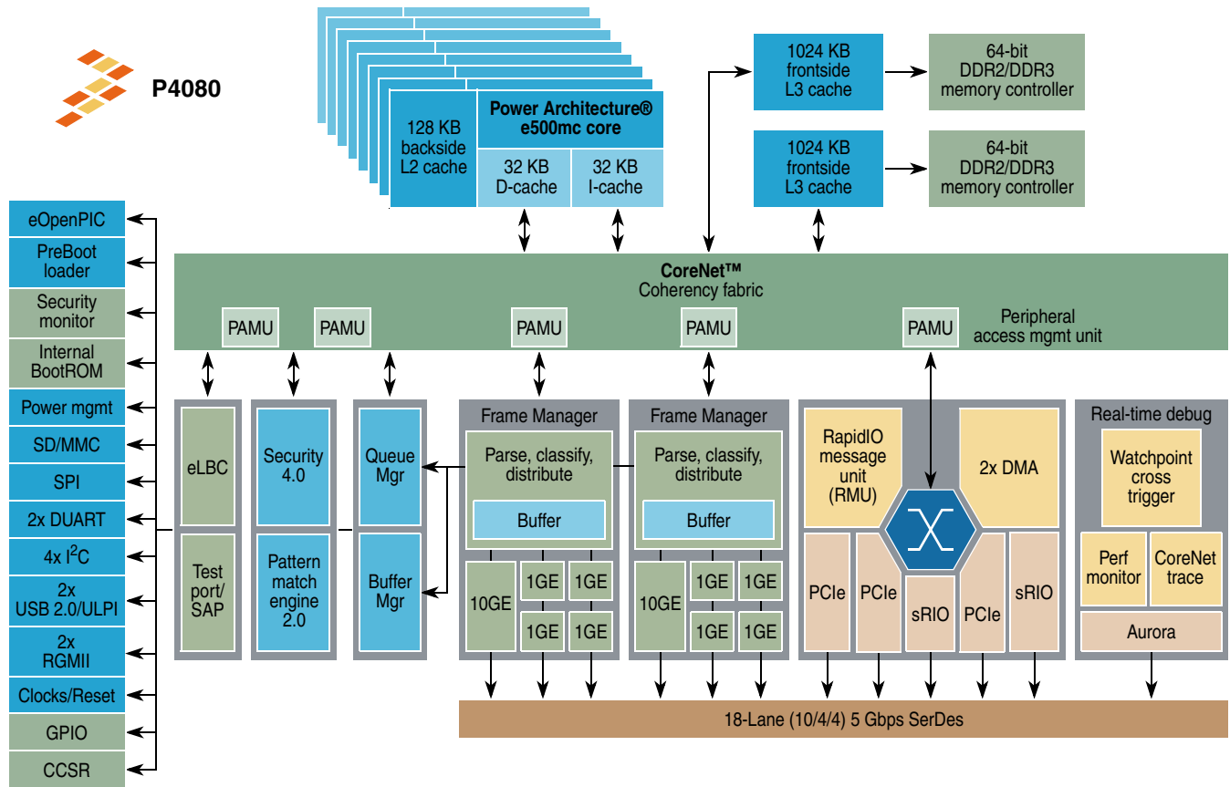
Figure 1. P4080 QorIQ Preliminary Block Diagram
