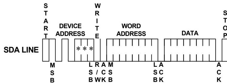
Figure 5: Byte Write
