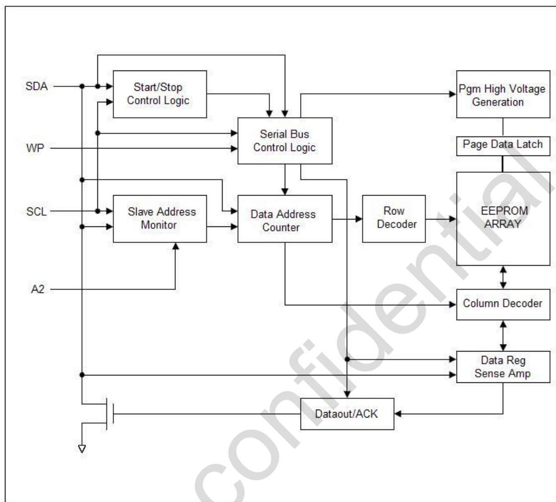
Figure 2: Block Diagram
