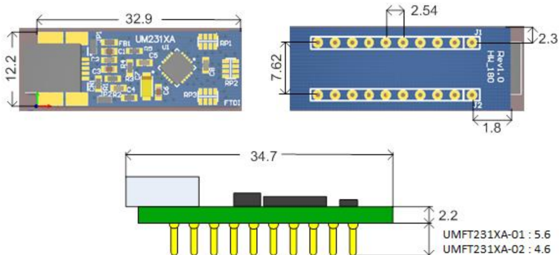
Figure 5.6 – UMFT231XA Module Dimensions
