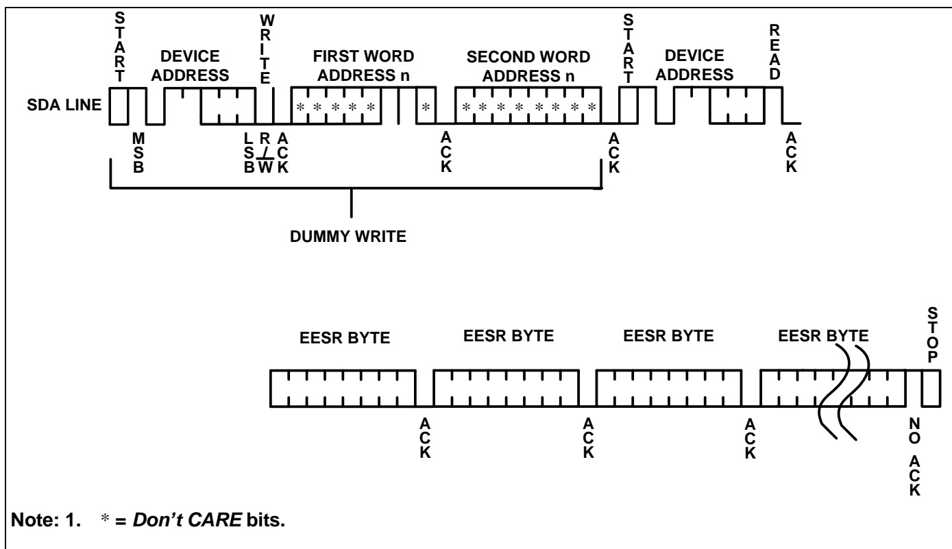
Figure 17. Read EESR
