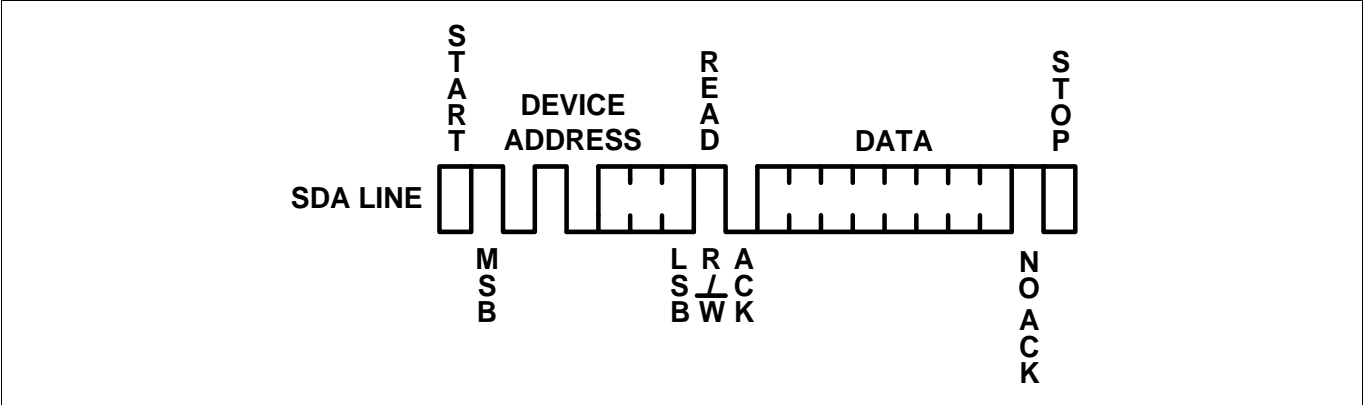
Figure 10. Random Read
