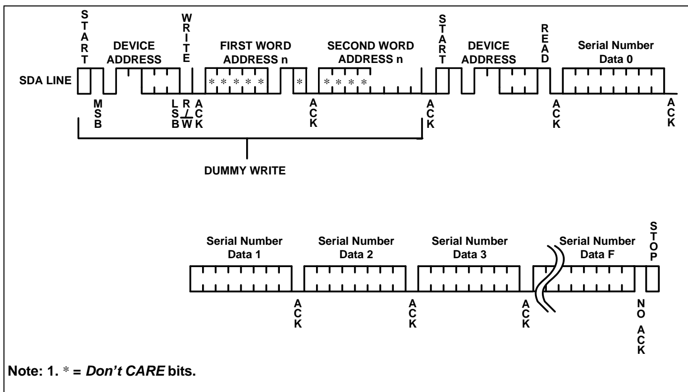
Figure 17. Read EESR
