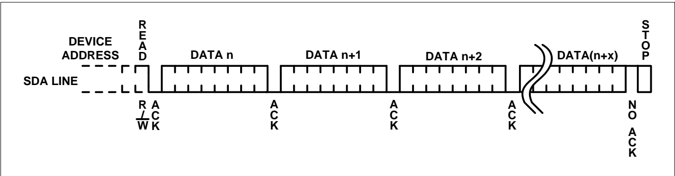
Figure 11. Sequential Read
