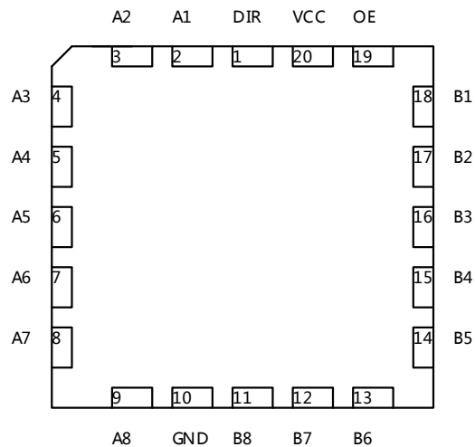
QFN20(4X4)
